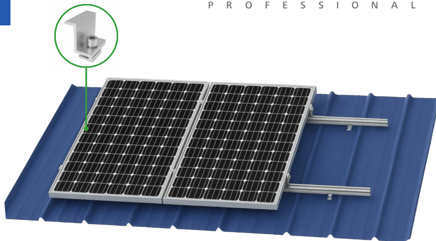
Terminal panel
